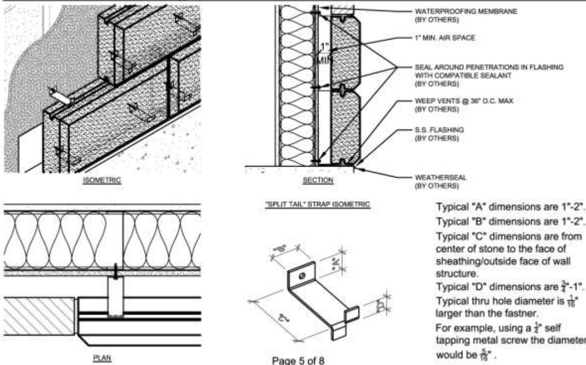
DETAIL 4-"SPLIT TAIL" STRAP @ VENEER
